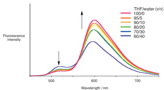
Figure 5. Fluorescence spectra of 1 in THF/water mixtures from 100:0 to 60:40 THF/H 2 O (v/v).
