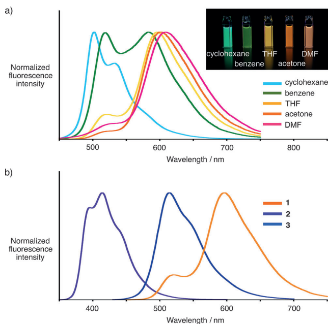
Figure 3. a) Fluorescence spectra of 1 in various solvents excited at 390 nm (inset: photographs under the irradiation with a 365 nm lamp) and b) fluorescence spectra of 1 , 2 , and 3 in THF (excitation wavelength: 390 nm for 1 and 3 , 330 nm for 2 ).
