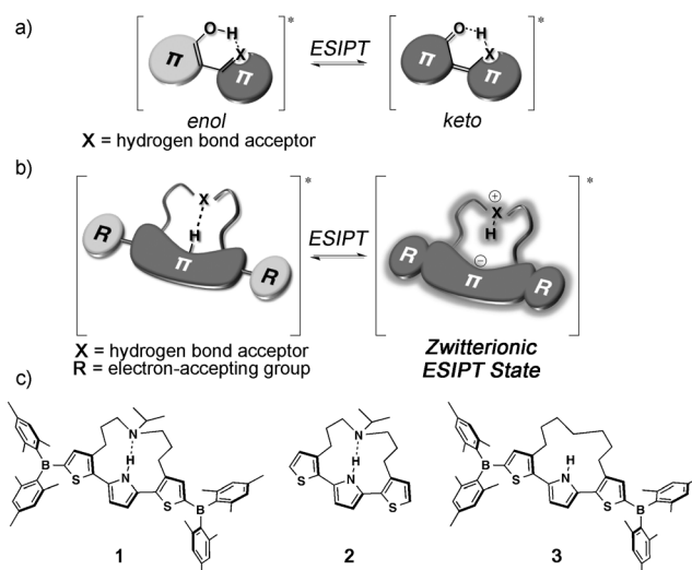
Figure 1. Designs of the excited-state proton transfer (ESIPT) systems based on a) a keto–enol type tautomerism and b) a strap strategy with a basic flexible chain. c) Chemical structures of compounds 1–3.
