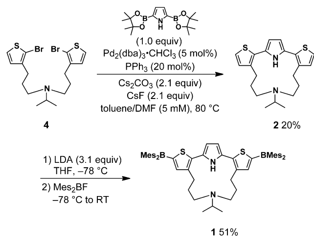
Scheme 1. Synthesis of compound 1 .
