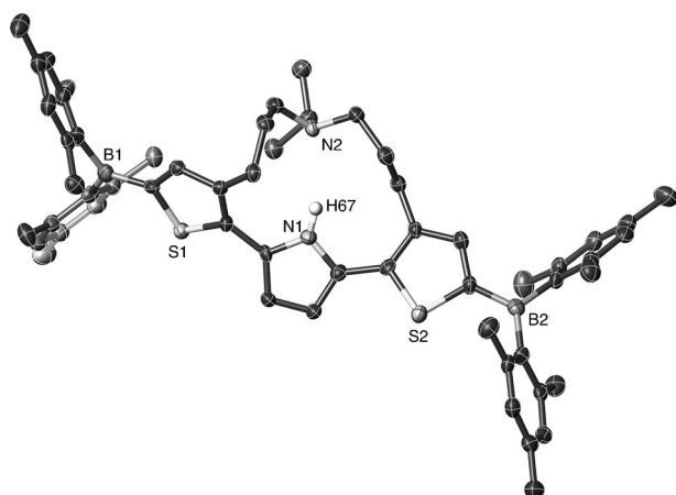
Figure 2. Thermal ellipsoid plot of 1 (50% probability). Hydrogen atoms are omitted for clarity except for the N–H proton on the pyrrole ring.
